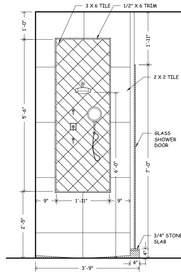
INTERIOR ELEVATION MASTER SHOWER Scale: 1/2" = 1'-0"
