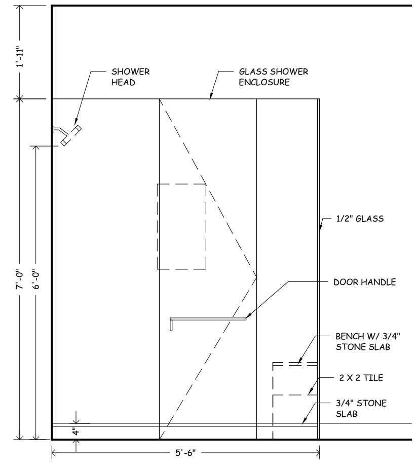
INTERIOR ELEVATION MASTER SHOWER Scale: 1/2" = 1'-0"
