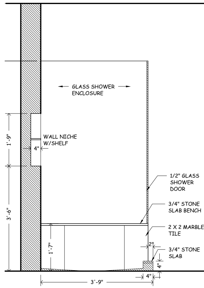
INTERIOR ELEVATION MASTER SHOWER Scale: 1/2" = 1'-0"
