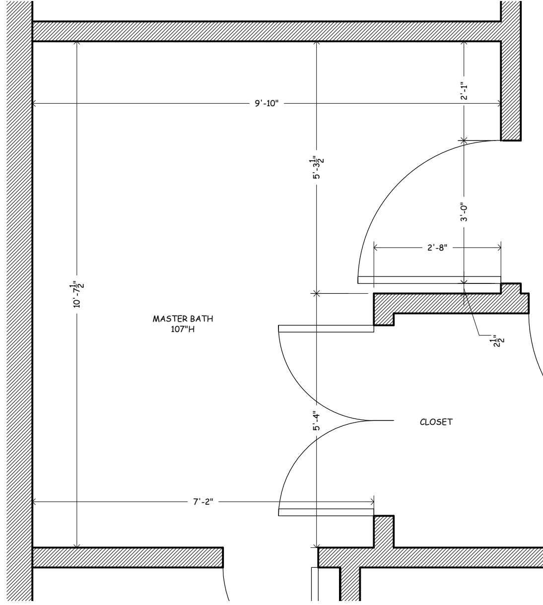
1 PARTIAL PROPOSED FLOOR PLAN FIRST LEVEL MASTER BATH Scale: 1/2" = 1'-0"
