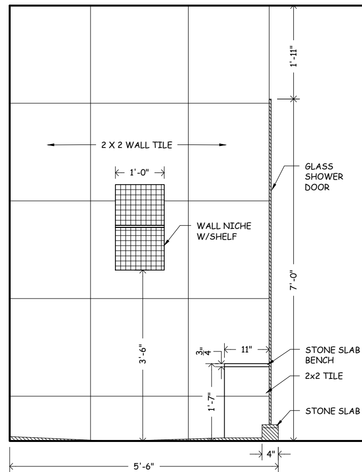
INTERIOR ELEVATION MASTER SHOWER Scale: 1/2" = 1'-0"
